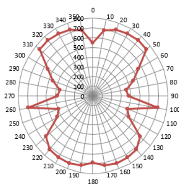
Wind Load @150 km/h
